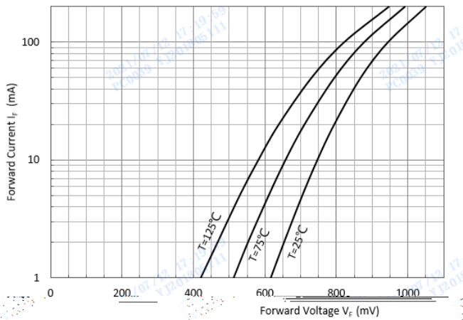
Forward Characteristics
